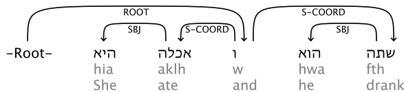
Figure 2: Coordinated Sentence
