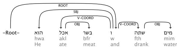
Figure 1: Coordinated Verbs
