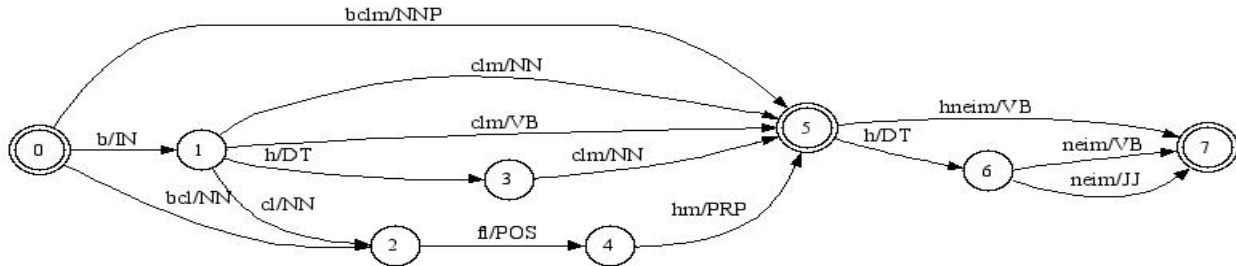
Figure 1: Lattice representation of the sentence bclm hneim . Double-circles denote token boundaries. Lattice arcs correspond to different segments of the token, each lattice path encodes a possible reading of the sentence. Notice how the token bclm have analyses which include segments which are not directly present in the unsegmented form, such as the definite article h (1-3) and the pronominal suffix which is expanded to the sequence fl hm (“of them”, 2-4, 4-5).
