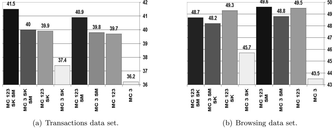
Figure 3: Exponential decay score for different Markov chain versions.
