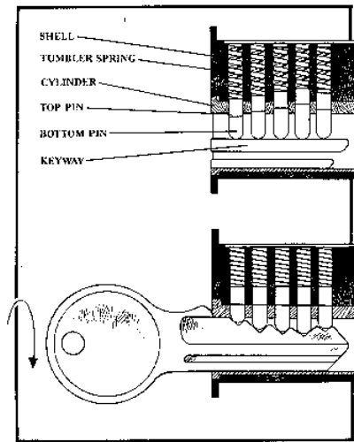
Figure 1. The pin tumbler lock, cutaway view.
