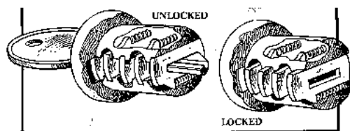
Figure 13. A wafer tumbler lock.
