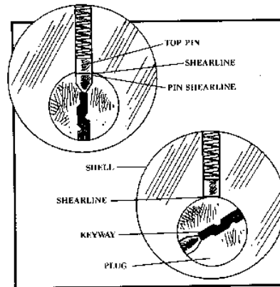
Figure 2. The pin tumbler lock, front view.
