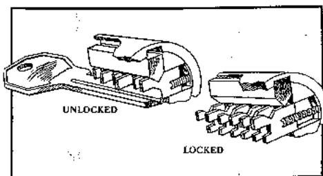
Figure 14. A side bar lock.
