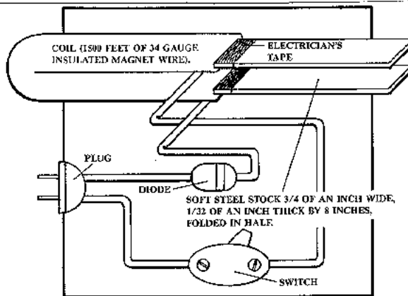
Figure 30. The magnetic pick is easy to construct.
