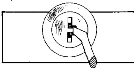
Figure 17. Inserting a tension wrench in a double-wafer lock.
