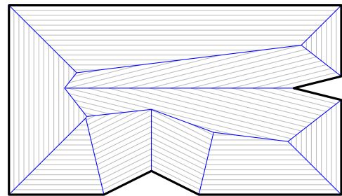
Figure 1: The straight skeleton \mathcal{S}(P) (blue) of the input polygon P (bold) is defined by the wavefront \mathcal{W}_P (gray) emanated from P .
