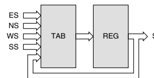
Figure 2. The rule table TAB and the state register REG of the automaton cell.
