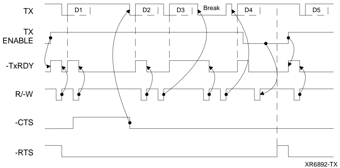
Figure 4: Transmit Timing
