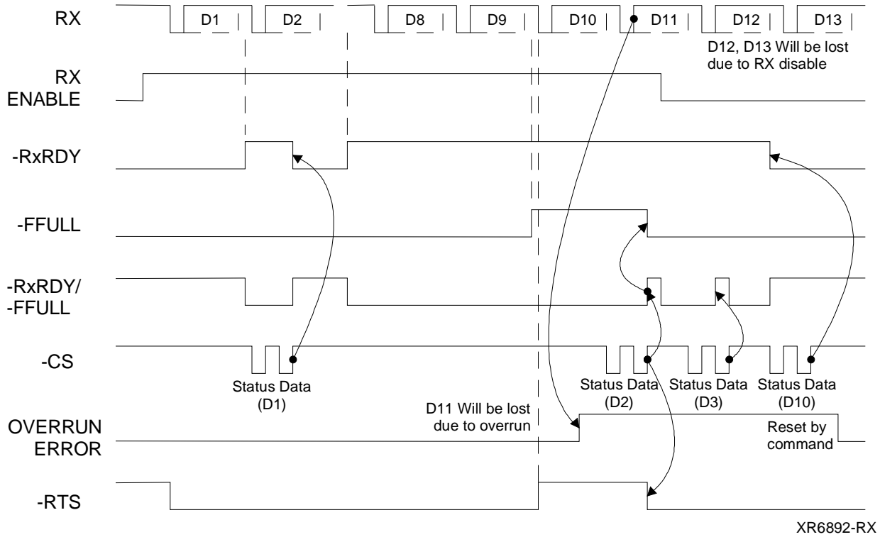
Figure 3: Receive Timing
