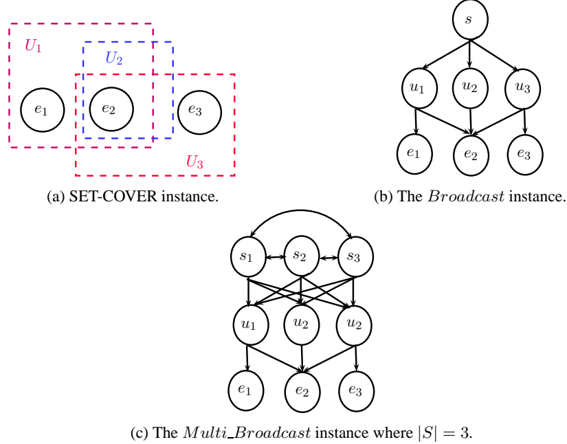
Figure 3: The reduction from SET-COVER to Broadcast and Multi-Broadcast .
