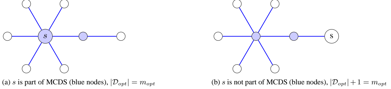
Figure 1: Similarity between MCDS and the optimal broadcast backbone. The value of m_{opt} denotes the size of optimal broadcast backbone, |\mathcal{D}_{opt}| denotes the size of optimal minimum connected dominating set and s is the source.
