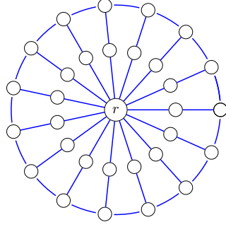
(a) Input graph G with d_G = 4
