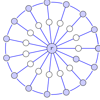
(b) MCDS (blue nodes) with |\mathcal{D}_{opt}| = 16 and d_D = 15
