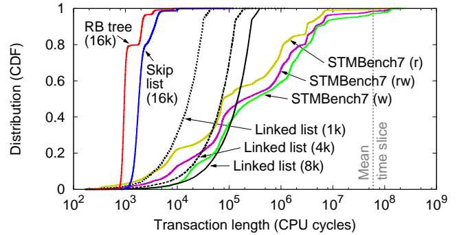
Figure 3. Transaction lengths for the synthetic benchmarks.
