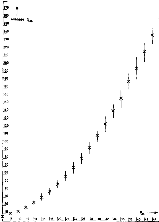
FIG. 1. Number of lines versus number of points for pseudorandomly generated graphs
