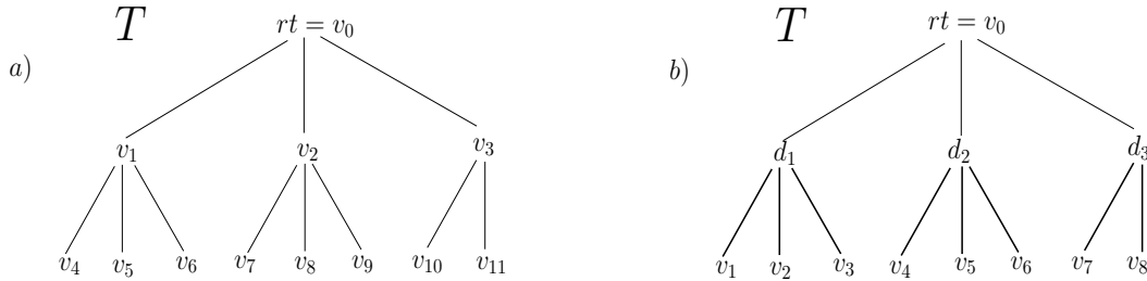
Figure 2: a) A 3-ary NSLoT for a 12-point metric space. b) A 3-ary Steiner NSLoT for a 9-point metric space M = (V, \text{dist}) . The Steiner points are d_1, d_2 and d_3 , and all other points rt = v_0, v_1, \dots, v_8 belong to the original point set V . Edges of weight \epsilon are depicted by thin lines. Edges of greater weight (specifically, edges (v_i, \pi(v_i)) of weight \text{dist}(rt, v_i) ) are depicted by bold lines.
