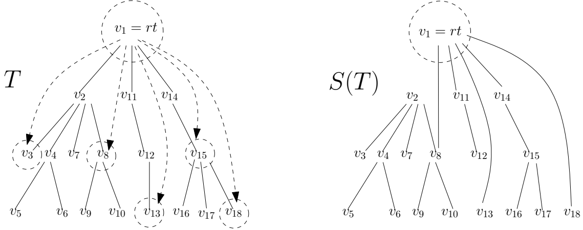
Figure 3: A spanning tree T of an 18-point metric space is depicted on the left. The vertices of T are ordered according to a pre-order traversal of T . The six breakpoints B_1 = v_1 , B_2 = v_3 , B_3 = v_8 , B_4 = v_{13} , B_5 = v_{15} and B_6 = v_{18} are enclosed within dashed circles. The edges in \mathcal{S} are depicted by dashed arrows. The graph \tilde{G} is obtained from T by adding to it all edges in \mathcal{S} . The tree S(T) , which is an SPT over \tilde{G} rooted at v_1 = rt , is depicted on the right. It contains only three out of the five edges in \mathcal{S} , and its root-degree is greater by two than the root-degree of T .
