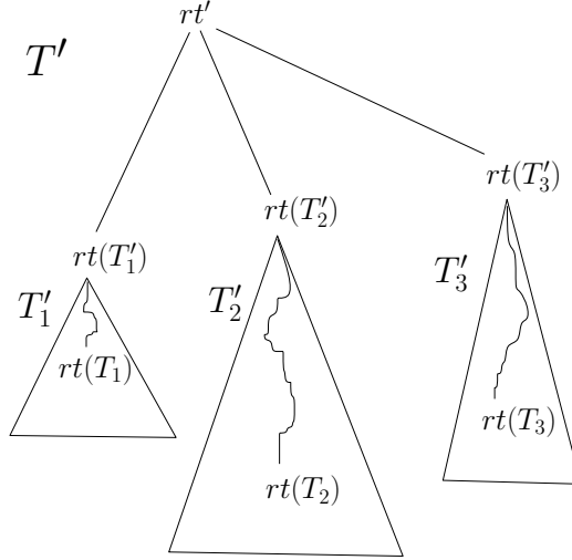
Figure 5: For every index i \in [3] , the vertex rt(T_i) belongs to the subtree T'_i of T' . Thus the path connecting rt' with rt(T_i) in T' passes through the vertex rt(T'_i) . Moreover, the required vertex closest to rt' in T' (excluding rt' itself if rt' \in R' ) is rt(T_1) .
