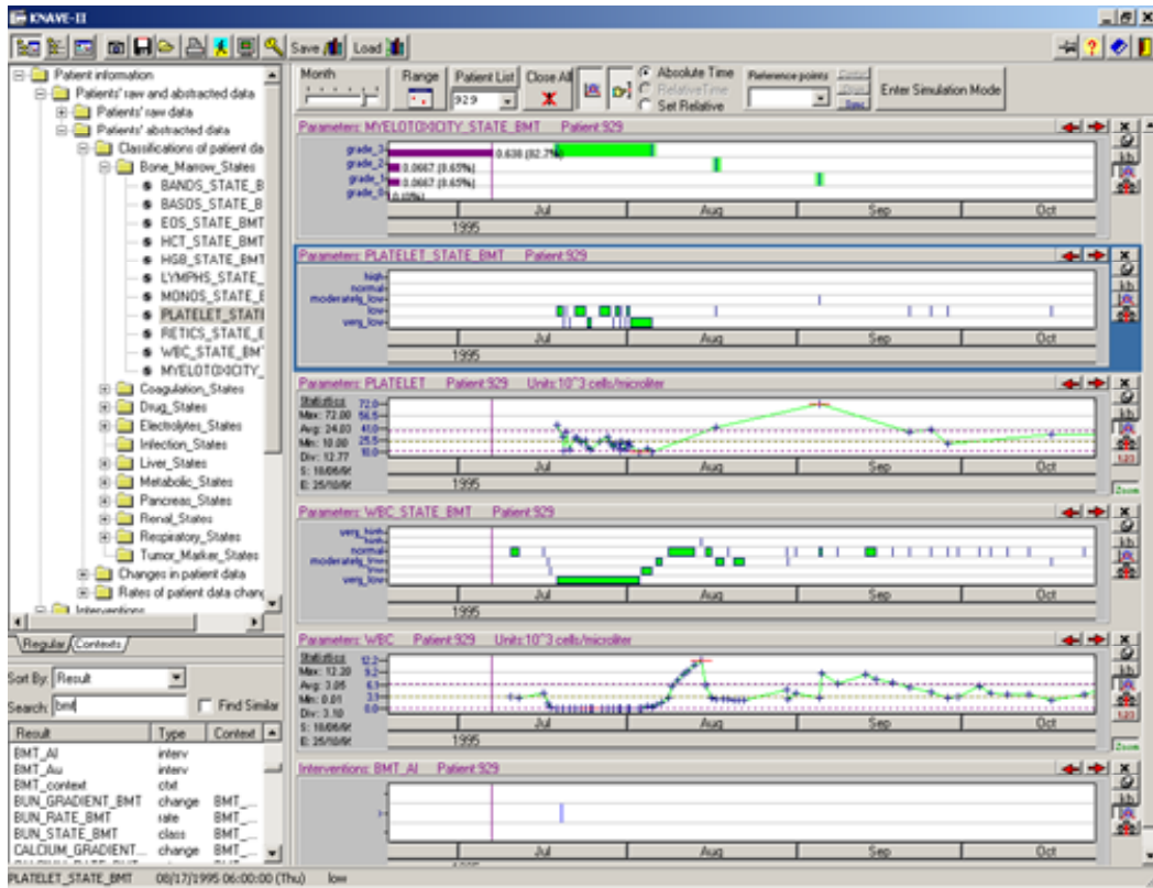
Fig. 5. The KNAVE-II main interface: This screen shows a view of an individual patient's data in an oncology domain. On the left hand side, a browser to the clinical domain's ontology, coming from the temporal abstraction knowledge source, is shown. The user selects a raw data (3rd, 5th and 6th panels from the top) or abstract concept (1st, 2nd and 4th)
