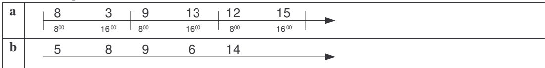
Fig. 3. Maximal sequences. The panels present sets of arbitrary measures. (a) The measures are performed every day at 8 and 16 o'clock. The set of constraints, C1 , constrains successive elements to be in gap of 24 hours, and with increasing values. There are two maximal sequences with respect to C1 : s1 = [8, 9, 12] and s2 = [3, 13, 15] . The sequences are disjoint, but overlapping in time. Note that the sequence [8, 9] is not maximal because the fact 12 can be added to the sequence without violating C1 . (b) The set of constraints, C2 , constrains successive elements to have increasing values. In this case there are two maximal sequences with respect to C2 : s3 = [5, 8, 9, 14] and s4 = [5, 6, 14] . In this case, the sequences are intersecting since the elements 5 and 14 appear in both. If the maximal sequence is specified as tight, the only sequences are s5 = [5, 8, 9] and s6 = [6, 14] . These sequences are disjoint and not overlapping in time.
