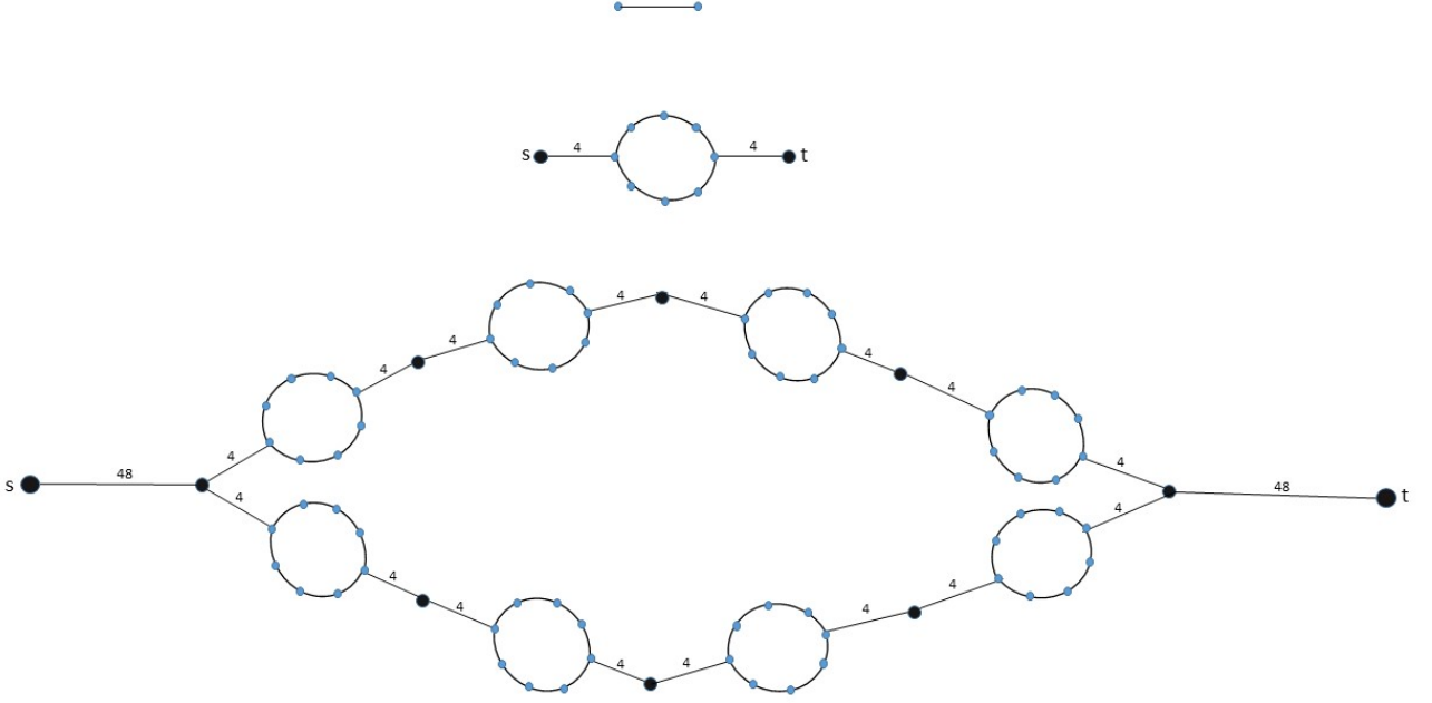
Figure 1: The first 3 levels of the recursive 4-cycle graph.
